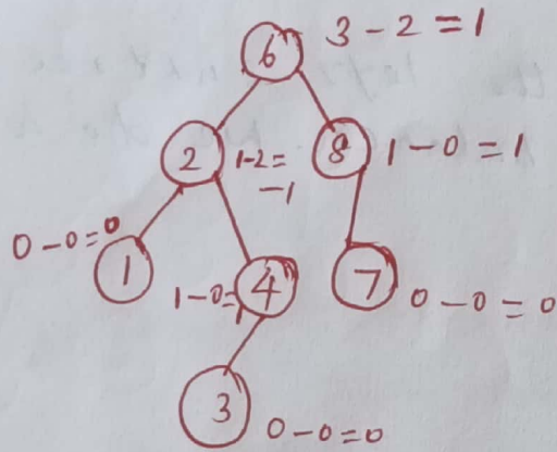
AVL Tree
