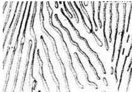
Figure 2.15 Pearlite
