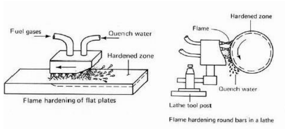
Figure 2.34 Flame hardening
