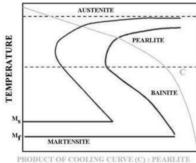
Figure 2.11 Slow cooling process (Annealing)
