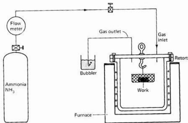
Figure 2.30 Nitriding process
