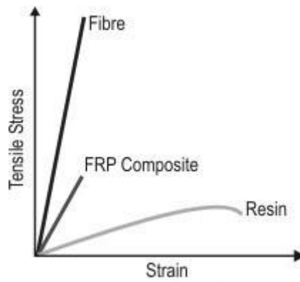
Figure 4.1 Illustrating the combined effect on Modulus of the addition of fibres to a resin matrix
