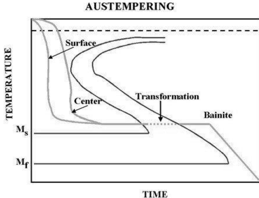
Figure 2.20 Austempering process.
