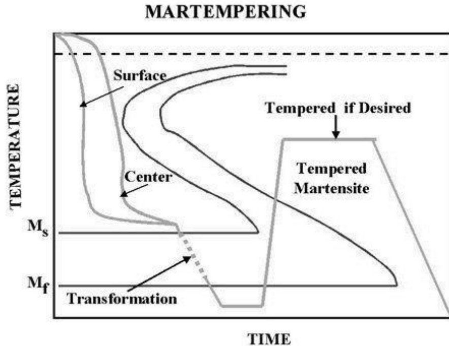
Figure 2.19 Martempering process.
