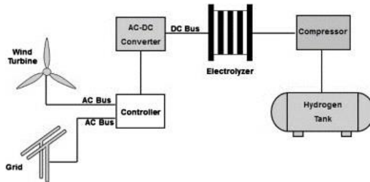
Fig. 28. Wind–hydrogen system
