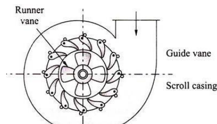
Fig. 26. Components of Kaplan turbine
