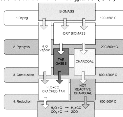
Fig.5. Gasification
