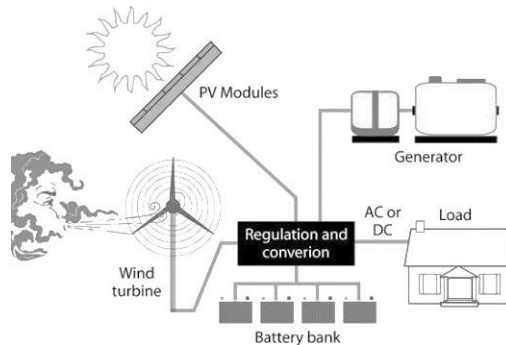
Fig. 26. Wind-solar hybrid system
