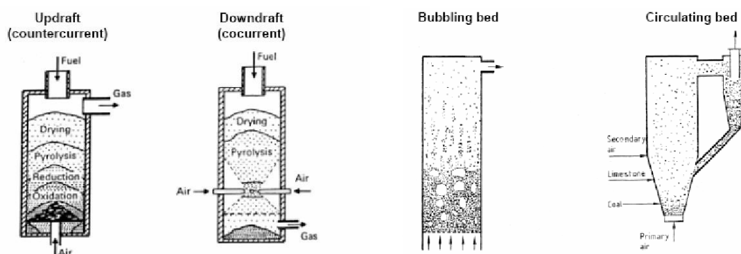
Fig1. Direct combustion processes
