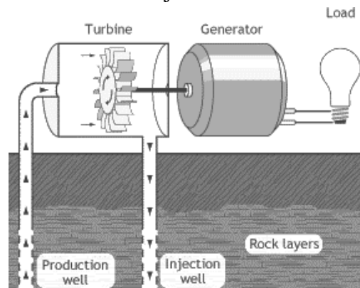
Fig. 17. Direct Dry Steam
