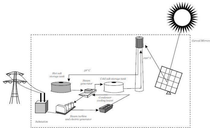
Fig.15. Operation of Central Receiver Power Plants
