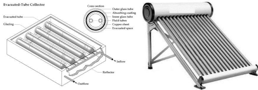
Fig. 10. Evacuated-Tube Collector
