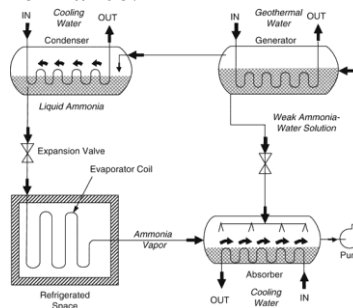
Fig.14. Refrigeration system
