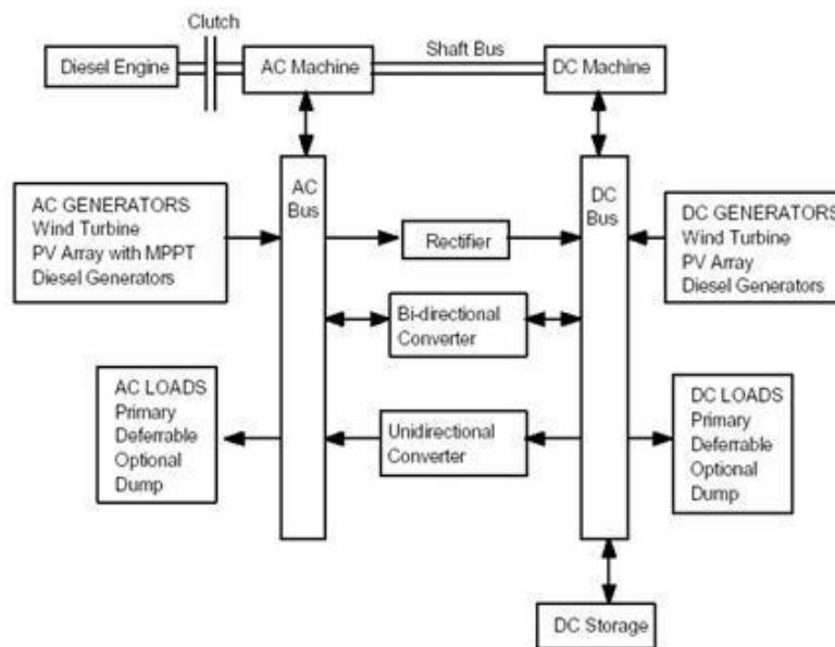
Fig. 25. Hybrid energy storage system
