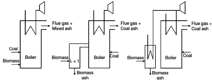
Fig.2. Cofiring
