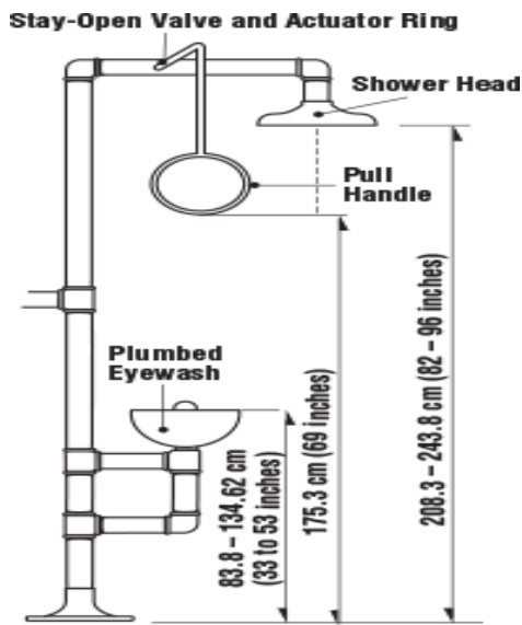
Fig.1 Shower Station
