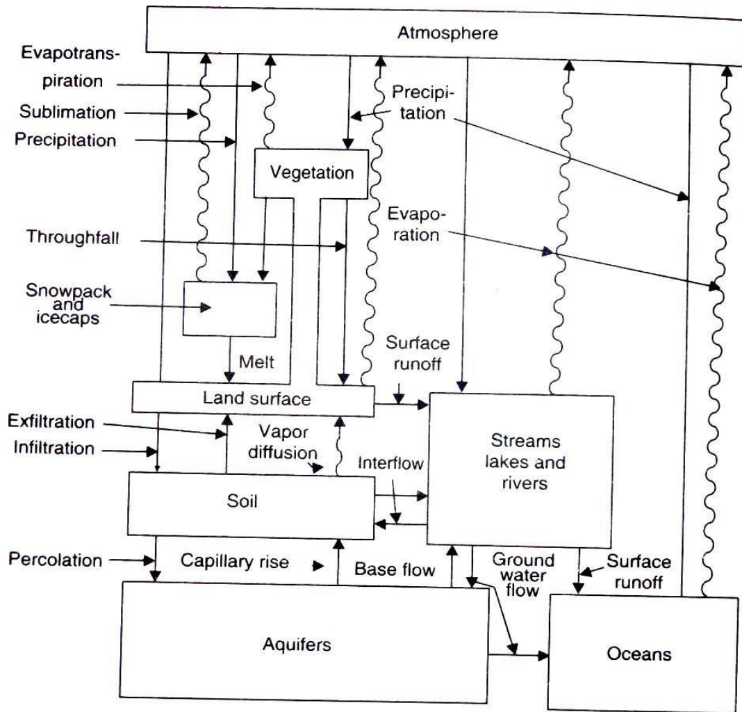
FIG1.3:Engineeringrepresentation ofHorton'shydrologicalCycle
