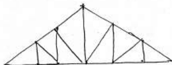
Howe - Triangle 6 panel. (12m to 24m span)
