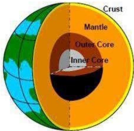
Fig- Inside the earth
