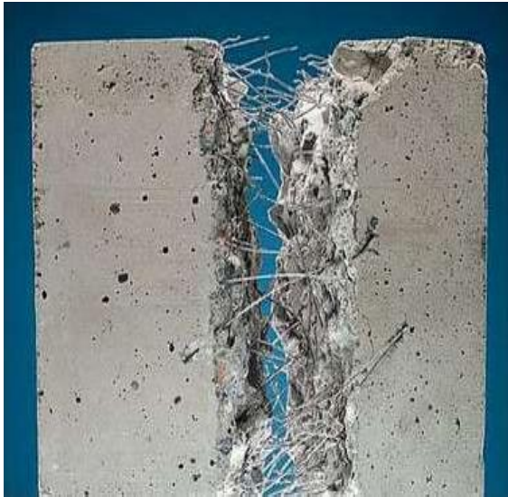
Fig- STEEL FIBERS
