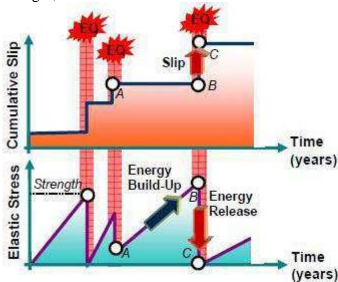
Fig- Elastic Rebound Theory
