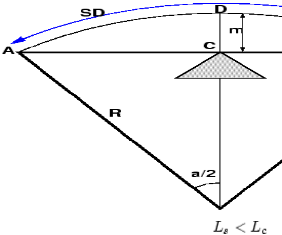
Figure 1: Set-back for single lane roads (
